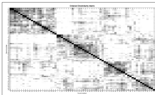
Figure 1. Axes are number of sound stimuli, gray scale correspond to percent of time that two sounds are grouped together. Black: 100% White: 0%
